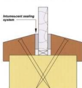
Typical Half Hour glazing system.
