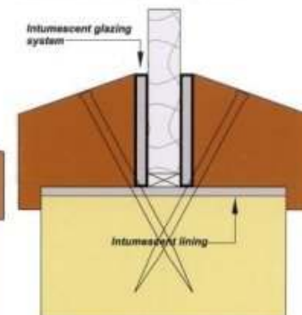
Typical one hour glazing system.
